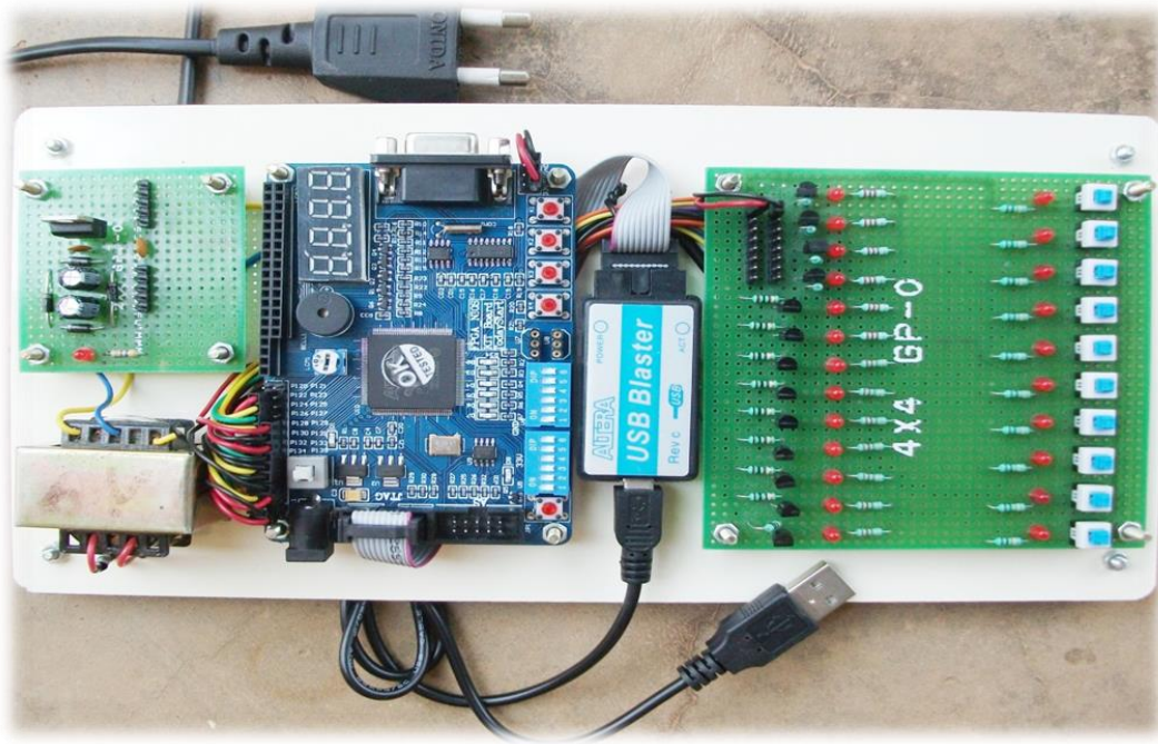
Altera Cyclone FPGA VLSI Trainer Kit by Dr. T. Veeramanikandaswamy of ECS
